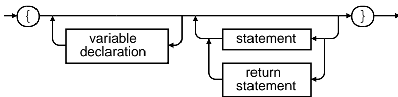
block:
