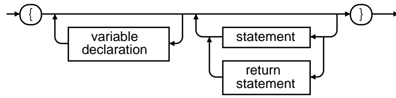
block:
