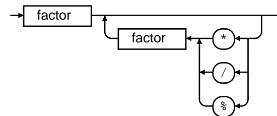
term:
