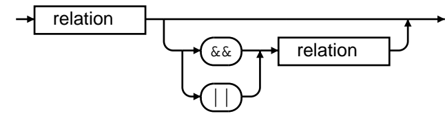
condition:
