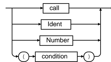
factor:
