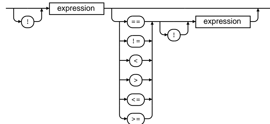
relation:
