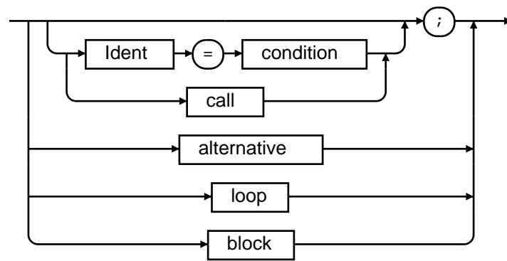
statement:
