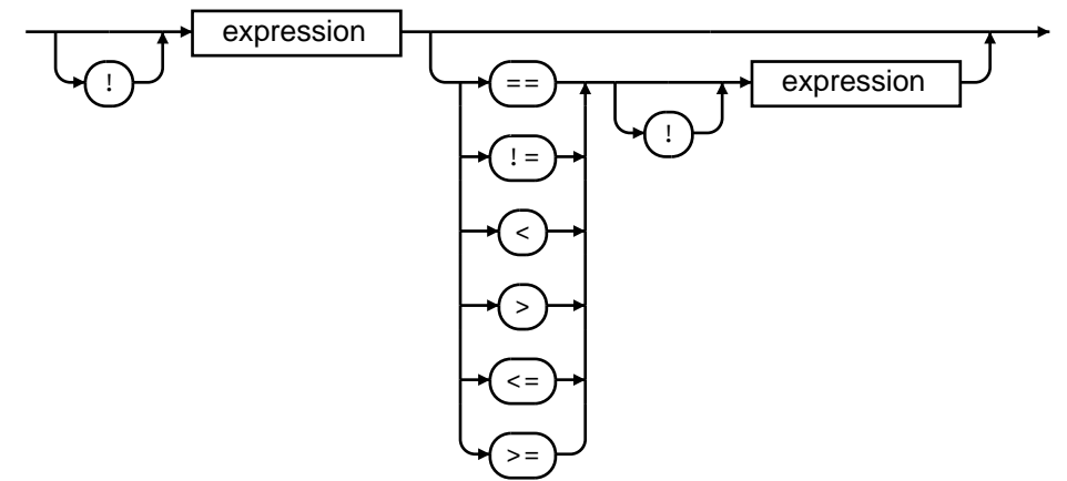
relation:
