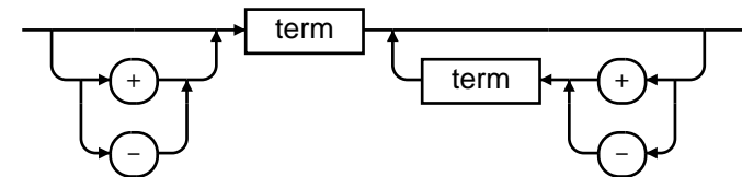
expression:
