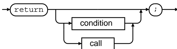
return-statement:
