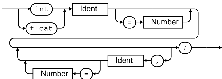
variable-declaration:
