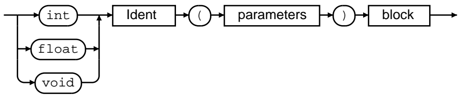
function-declaration:
