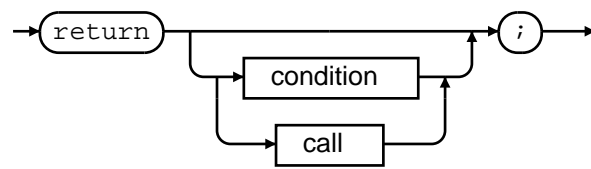
return-statement:
