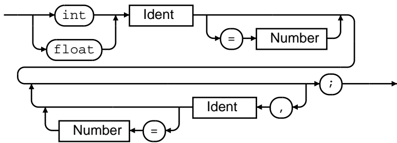
variable-declaration:
