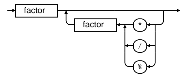
term:
