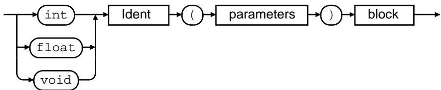
function-declaration:
