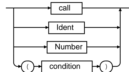
factor:
