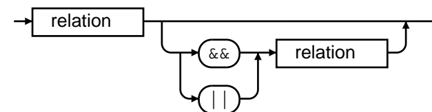
condition:
