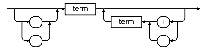
expression:
