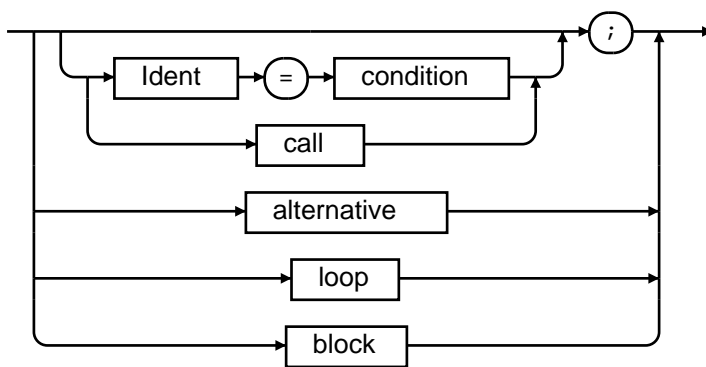
statement:
